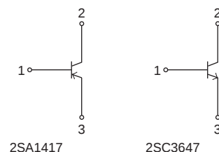
2SA1417
